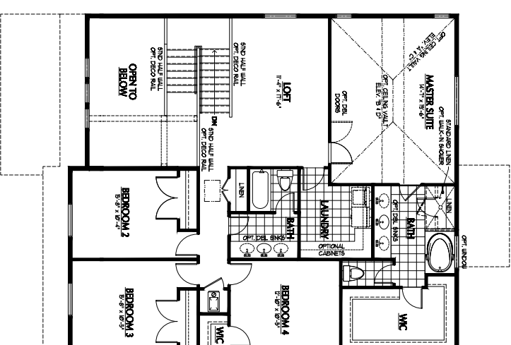
SECOND FLOOR (8'-0" STND CEILINGS)
