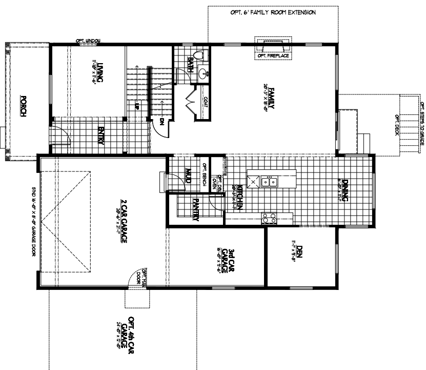
MAIN FLOOR (9'-0" STND CEILINGS)
