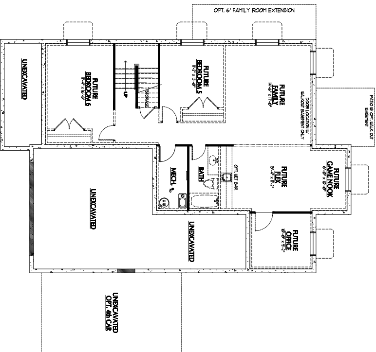
BASEMENT (8'-0" STND CEILINGS)
