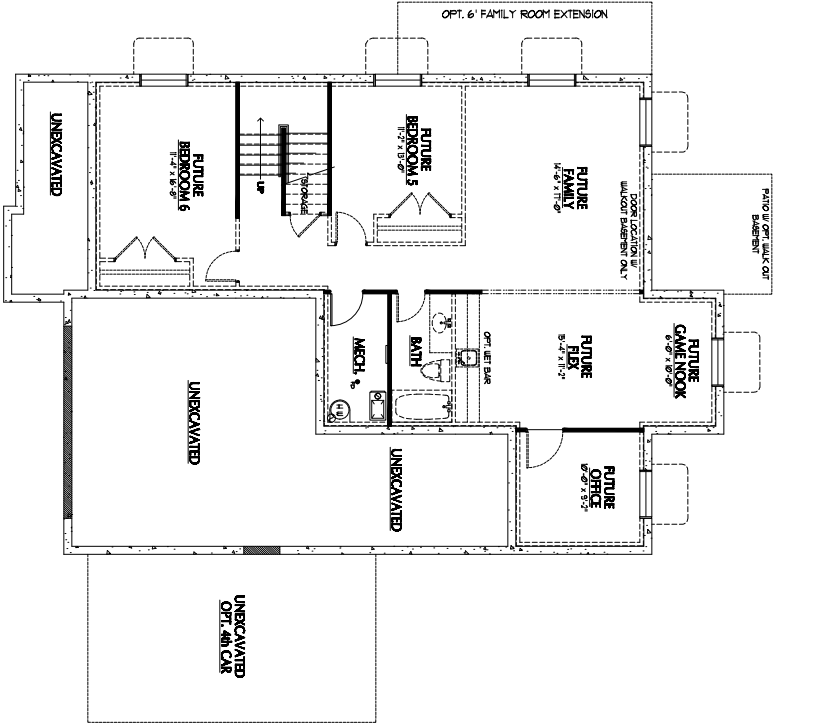
BASEMENT (8'-0" STND CEILINGS)
