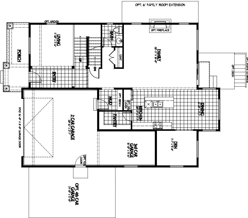
MAIN FLOOR (9'-0" STND CEILINGS)
