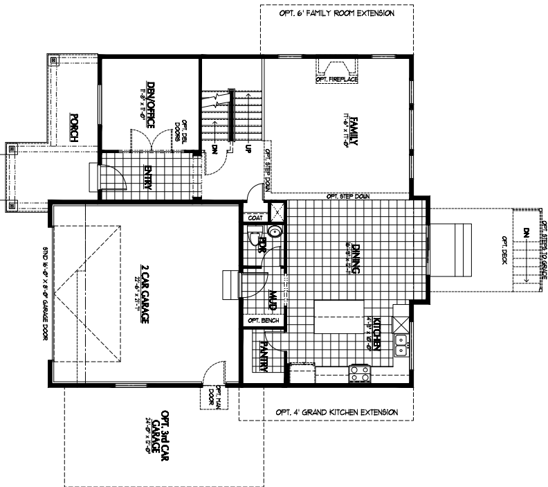
MAIN FLOOR (9'-0" STND CEILINGS)
