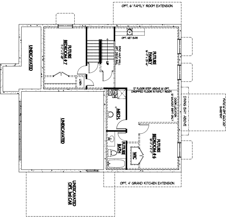
BASEMENT (8'-0" STND CEILINGS)
