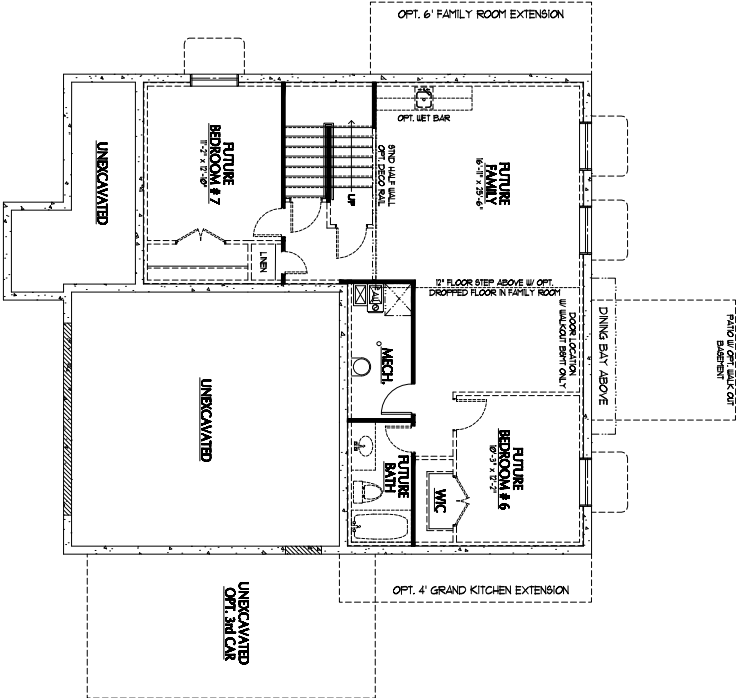
BASEMENT (8'-0" STND CEILINGS)
