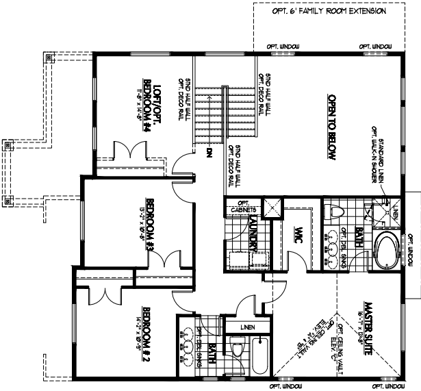
SECOND FLOOR (8'-0" STND CEILINGS)
