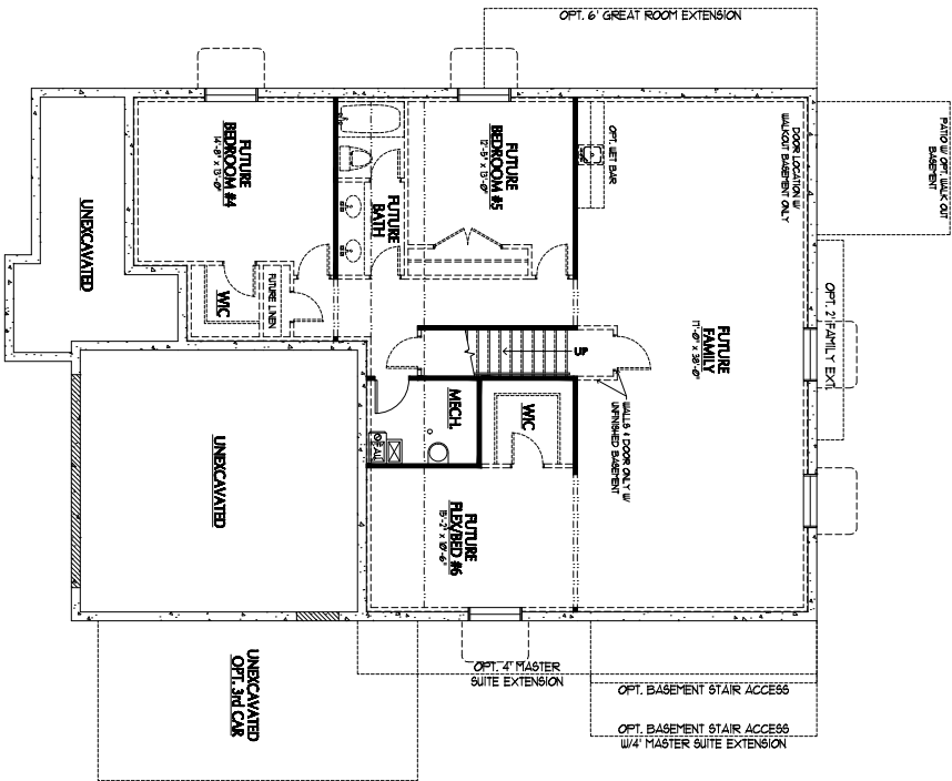
BASEMENT (8'-0" STND CEILINGS)
