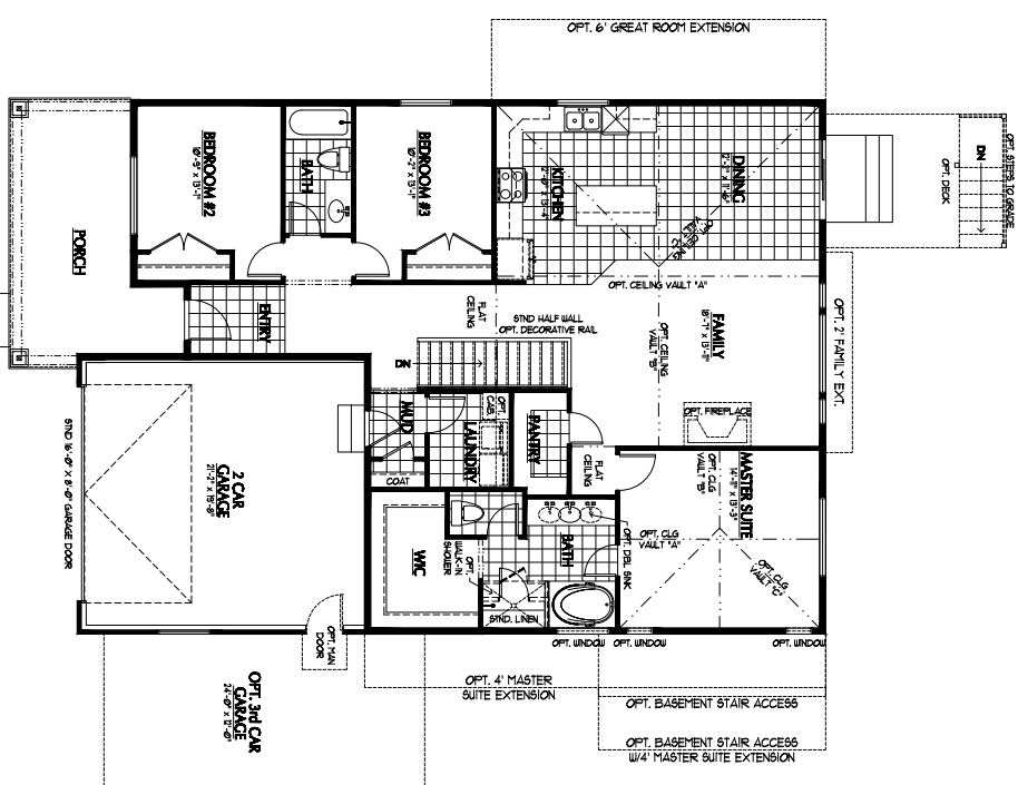
MAIN FLOOR PLAN (9'-0" STND CEILINGS)
