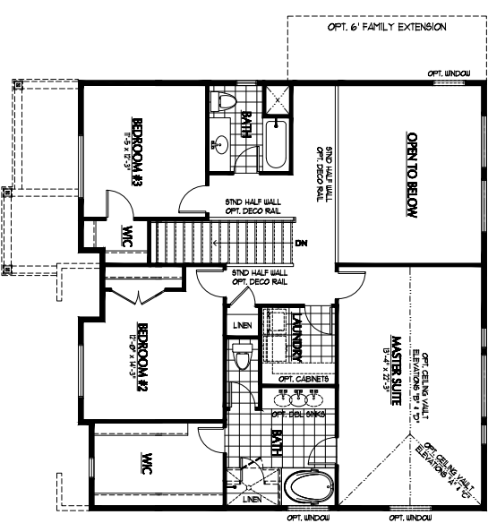
SECOND FLOOR (8'-0" STND CEILINGS)
