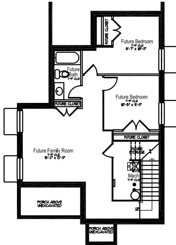
BASEMENT FLOOR
