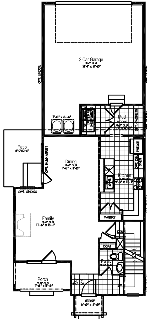
FIRST FLOOR
