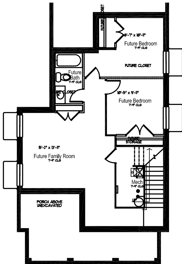
BASEMENT FLOOR
